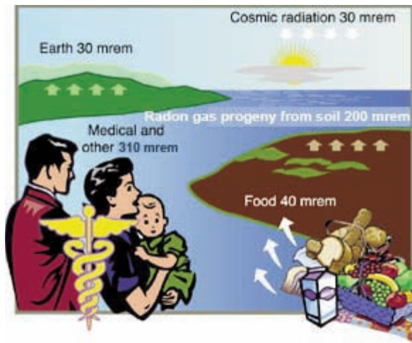
Figure 1. Annual Radiation Doses in the United States from Natural and Manufactured Radiation Sources. 1
